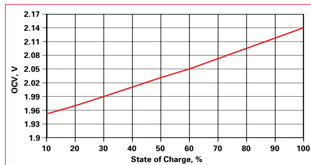
Figure 5-1: CYCLON Open Circuit Voltage Vs. State of Charge
