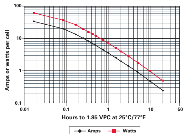
Figure A-10: 5.0Ah Single Cell Discharge to 1.85 VPC
