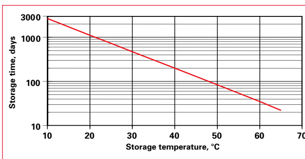
Figure 5-2: CYCLON Storage Time Vs. Temperature
