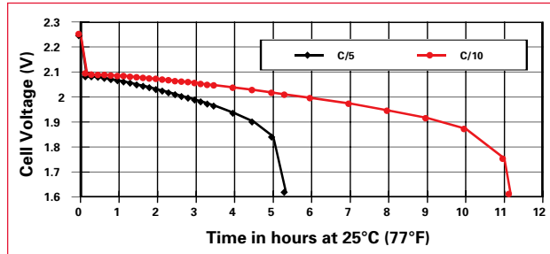
Figure 4-2: CYCLON High Rate Voltage Profile
