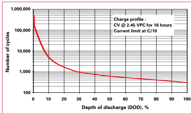
Figure 7-1: Cycle Life and DOD for CYCLON Cells
