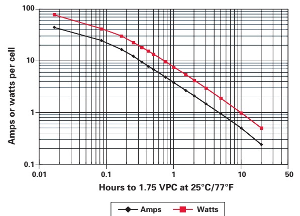
Figure A-9: 5.0Ah Single Cell Discharge to 1.75 VPC
