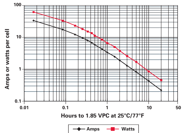
Figure A-8: 4.5Ah Single Cell Discharge to 1.85 VPC
