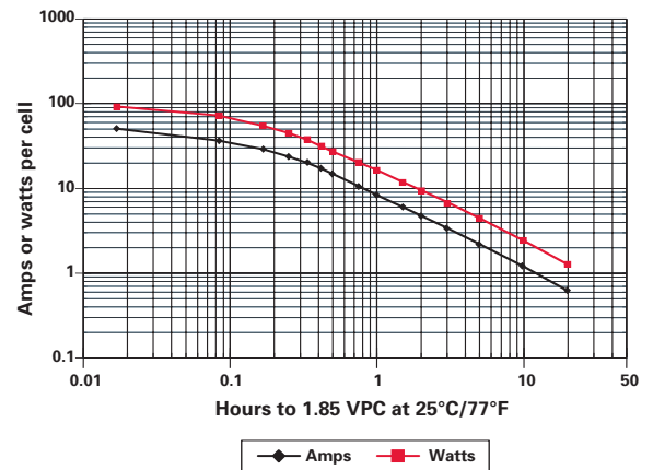
Figure A-14: 12.0Ah Single Cell Discharge to 1.85 VPC
