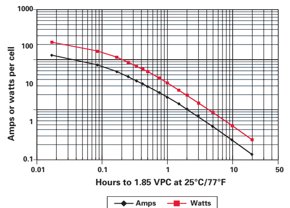
Figure A-16: 25.0Ah Single Cell Discharge to 1.85 VPC
