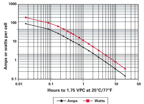
Figure A-15: 25.0Ah Single Cell Discharge to 1.75 VPC
